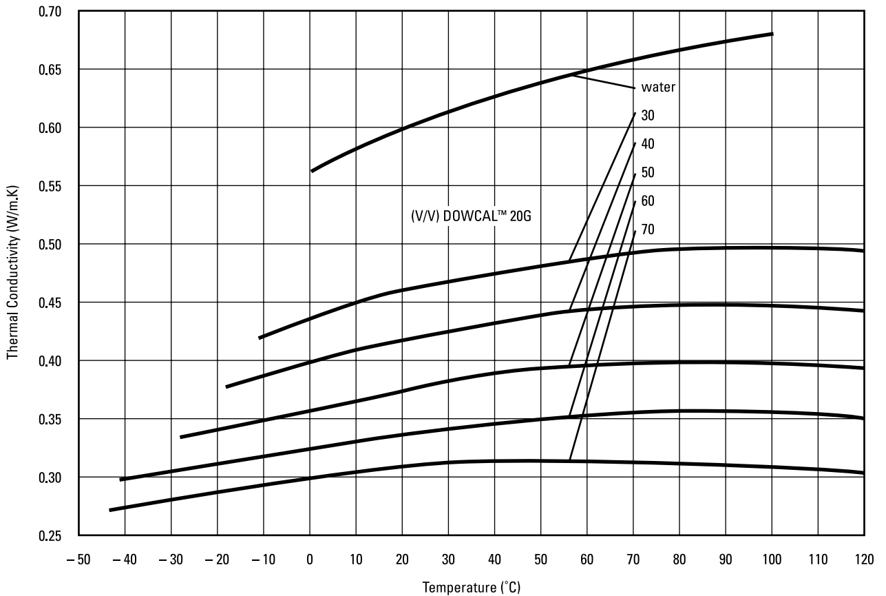
Figure 10 Thermal conductivity of aqueous solutions of DOWCAL™ 20G Fluid
