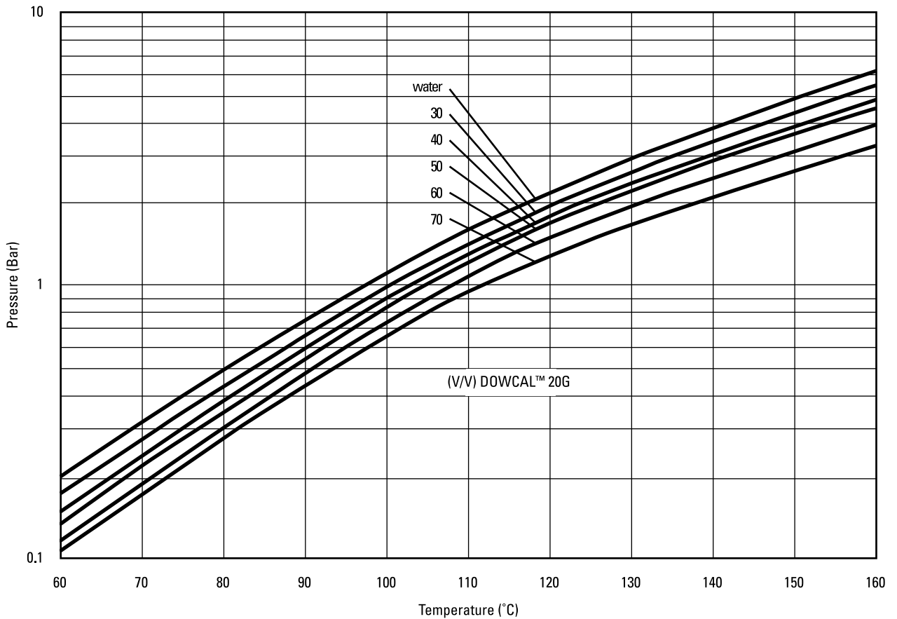
Figure 4 Vapour pressure over aqueous solutions of DOWCAL™ 20G
