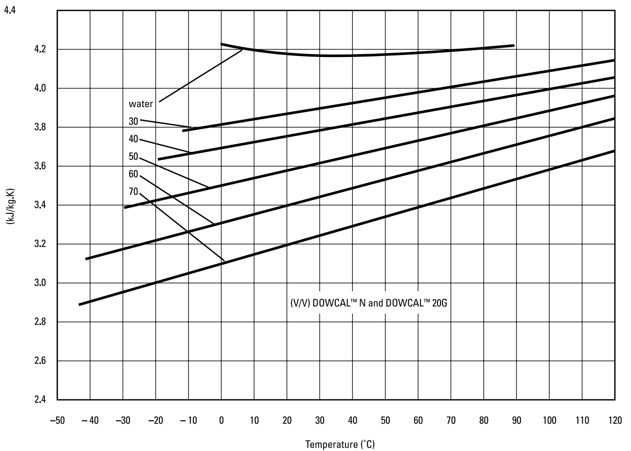
Figure 12 Specific heat of aqueous solutions of DOWCAL™ N and DOWCAL™ 20G Fluids
